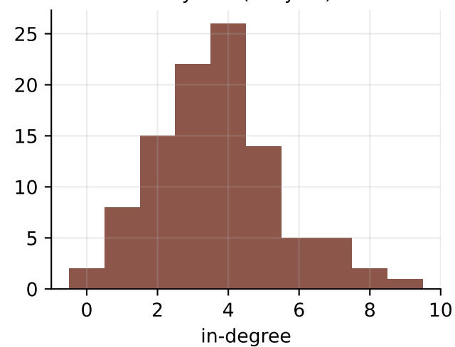
Layered (3 layers)
